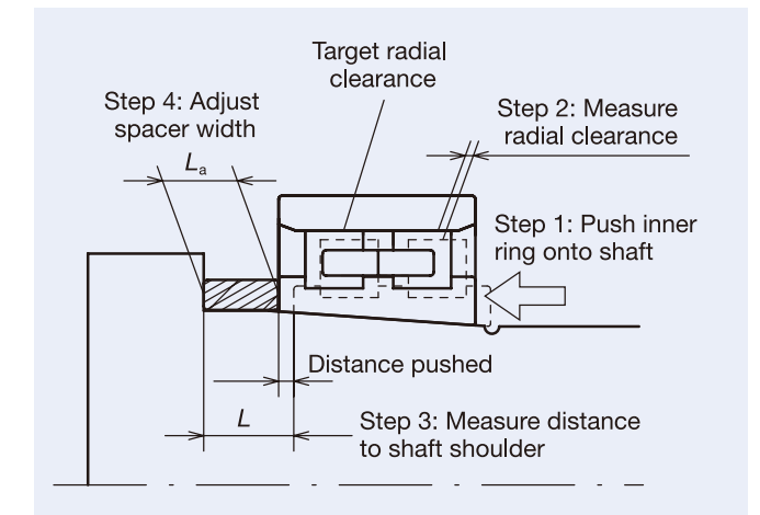
Fig. 1.4 Adjusting the Radial Clearance of Cylindrical Roller Bearings
