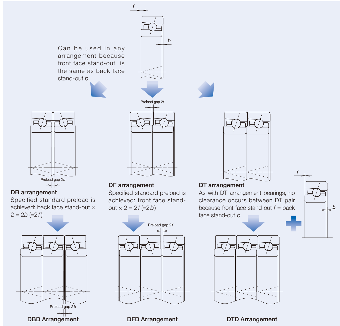
Fig. 3.9 Universal Arrangement
