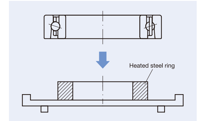
Fig 1.27 Heating the Inner Ring by means of a Hot Plate
