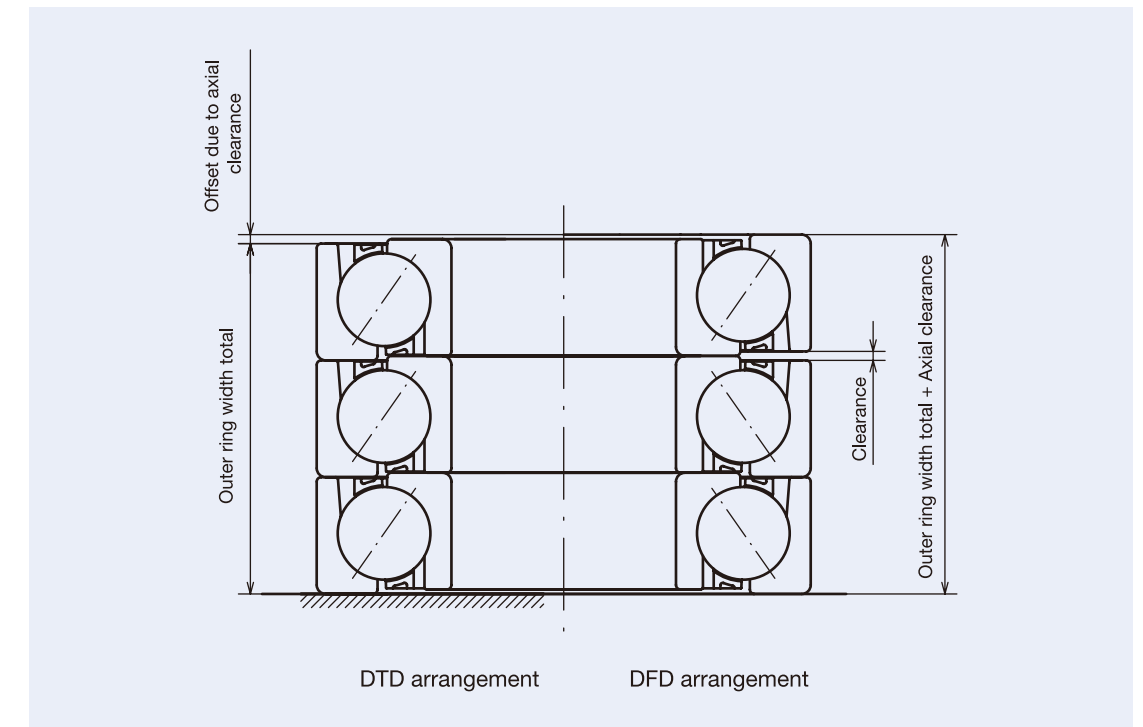
Fig. 1.21 Influence of Arrangement Type on Measurement of Outer Ring Width Total
