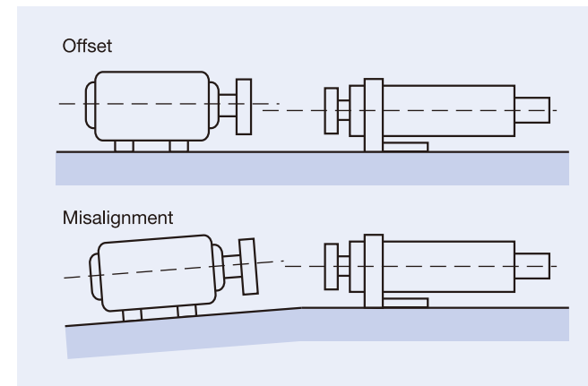
Fig. 2.2 Coupling Drive
