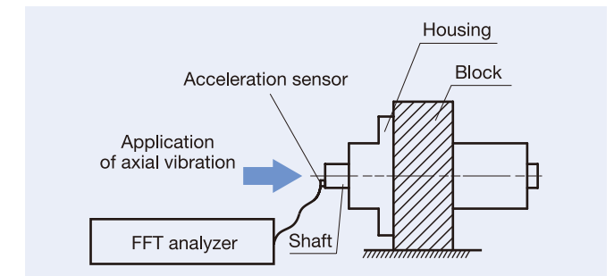
Fig. 1.37 Natural Frequency Method
