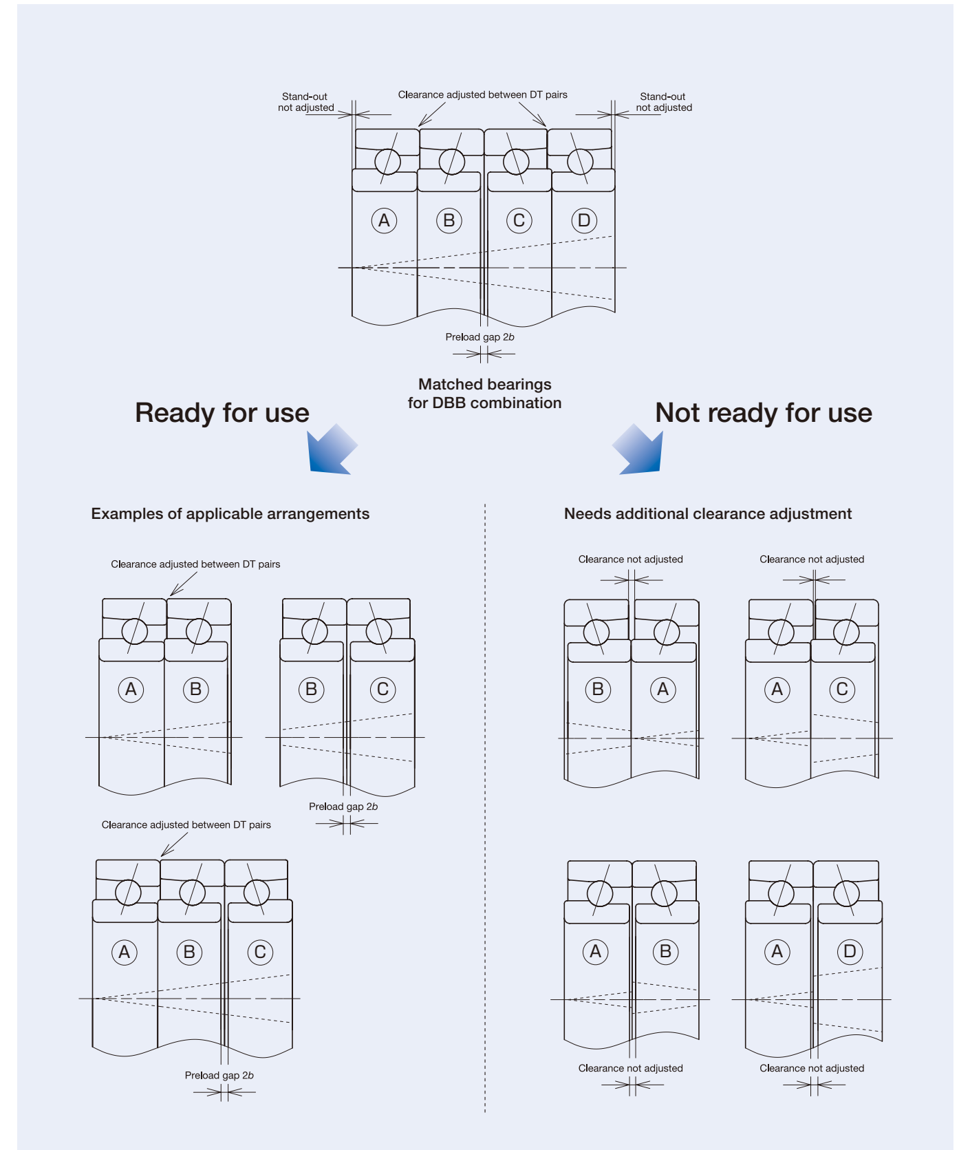
Fig. 3.8 DBB Combination
