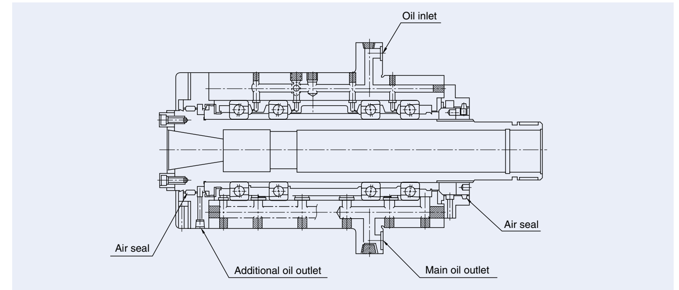
Fig. 6.5 Jet Lubrication Spindle (Example)
