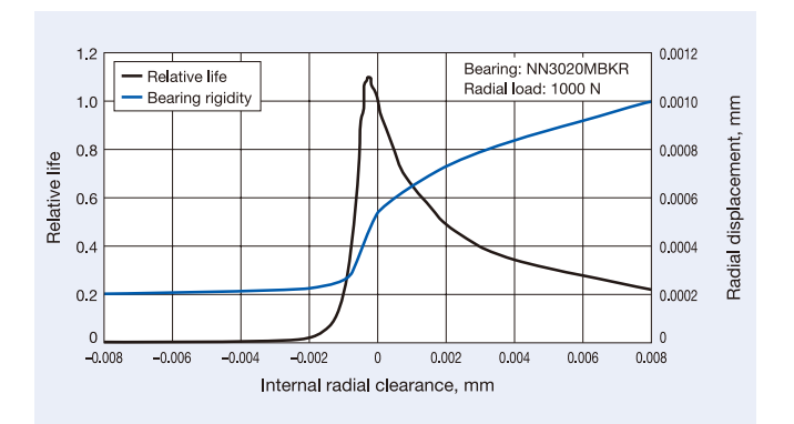
Fig. 4.9 Influence of Internal Radial Clearance on Rolling Fatigue Life and Rigidity in a Double-Row Cylindrical Roller Bearing
