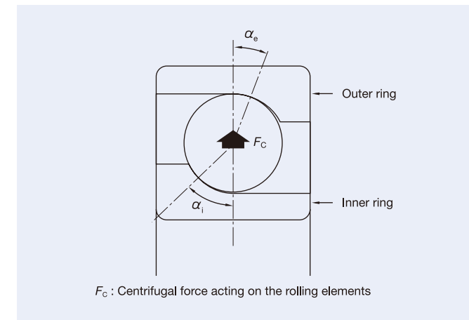
Fig. 1.7 Change in Contact Angle Due to Centrifugal Force
