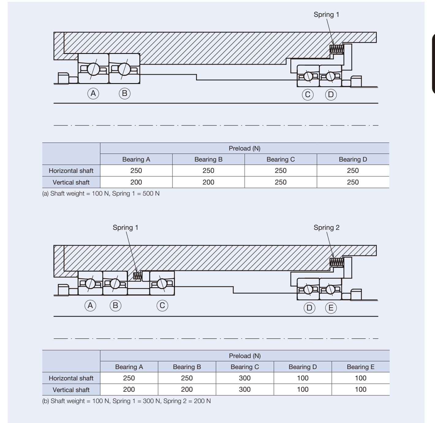
Fig. 4.6 Distribution of Preload in Constant Pressure Preload
