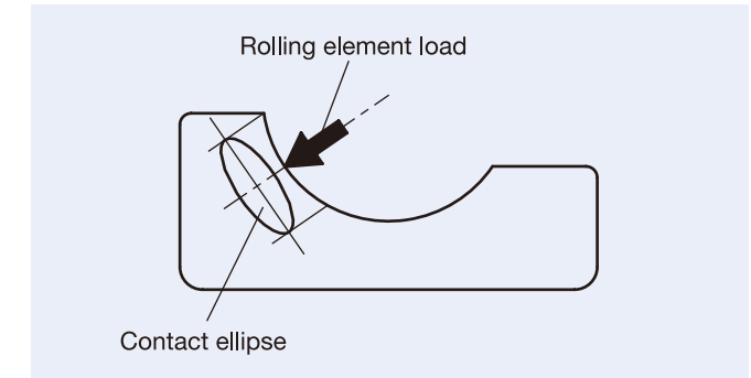
Fig. 2.2 Limiting Axial Load in Terms of Surface Pressure
