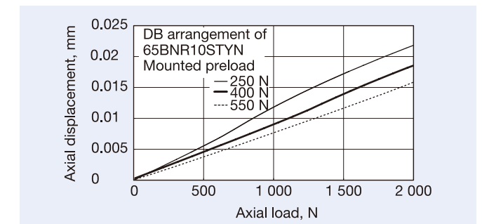
Fig. 1.36 Relationship between Axial Displacement and Preload
