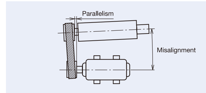
Fig. 2.1 V-belt Drive
