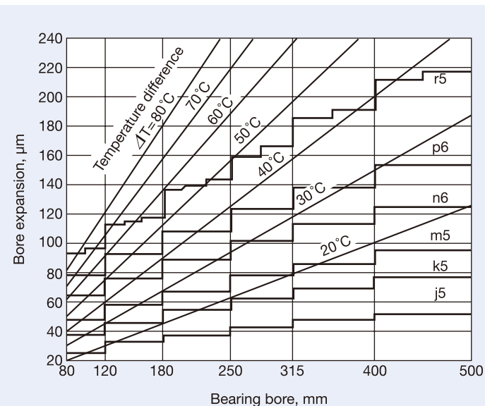
Fig 1.25 Temperature and Thermal Expansion of Inner Ring
