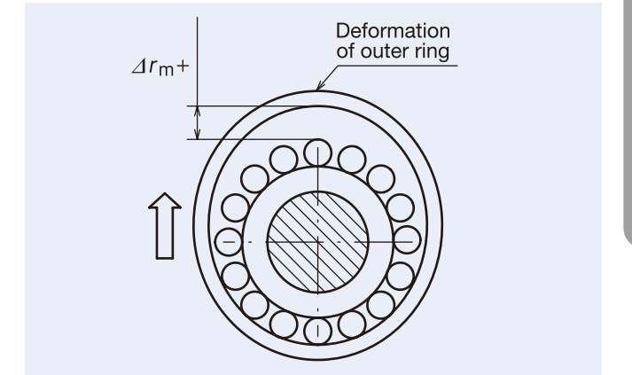
Fig 1.15 Deformation of the Outer Ring Due to Measuring Force
