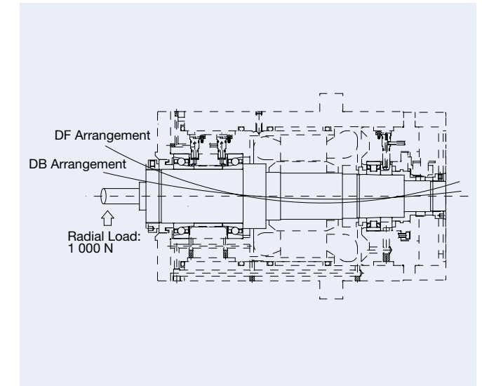
Fig. 3.4 Spindle Deflection Curve
