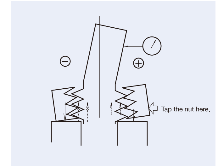
Fig 1.31 Adjusting Misaligned Shaft Locknut
