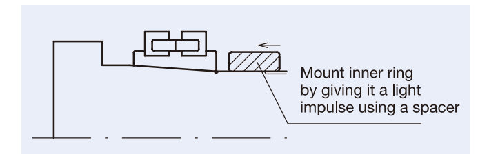
Fig. 1.5 Pushing the Inner Ring in Place
