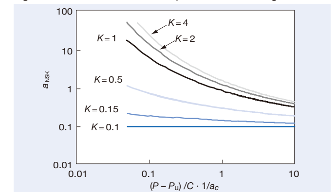
Fig. 1.5 New Life Calculation Graph for Roller Bearings
