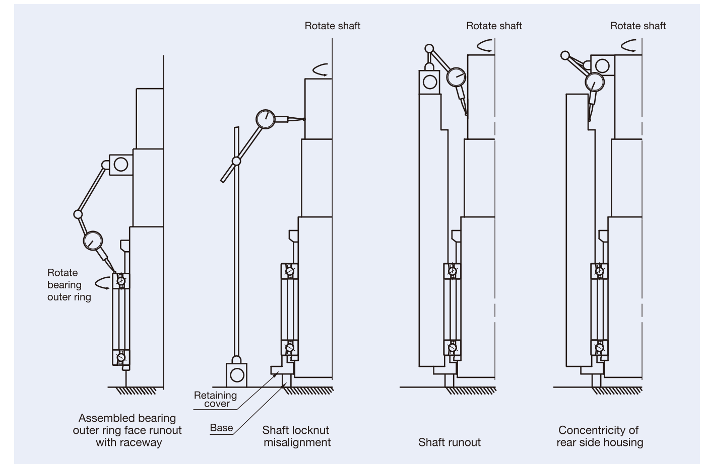
Fig 1.32 Measuring Spindle Runout
