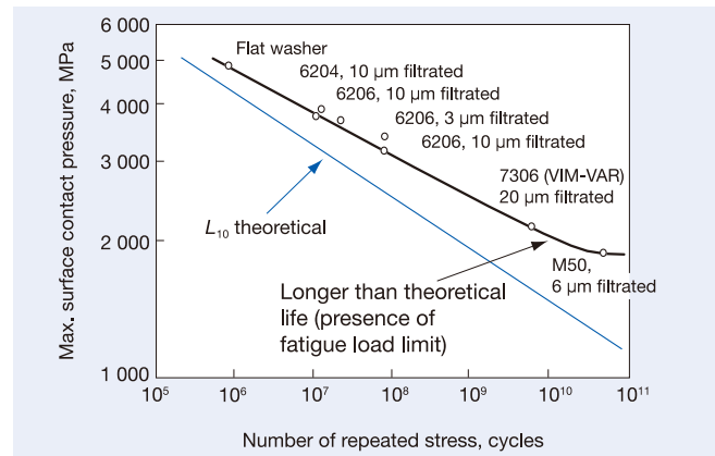
Fig. 1.2 Life Test Results Under Clean Lubrication Conditions
