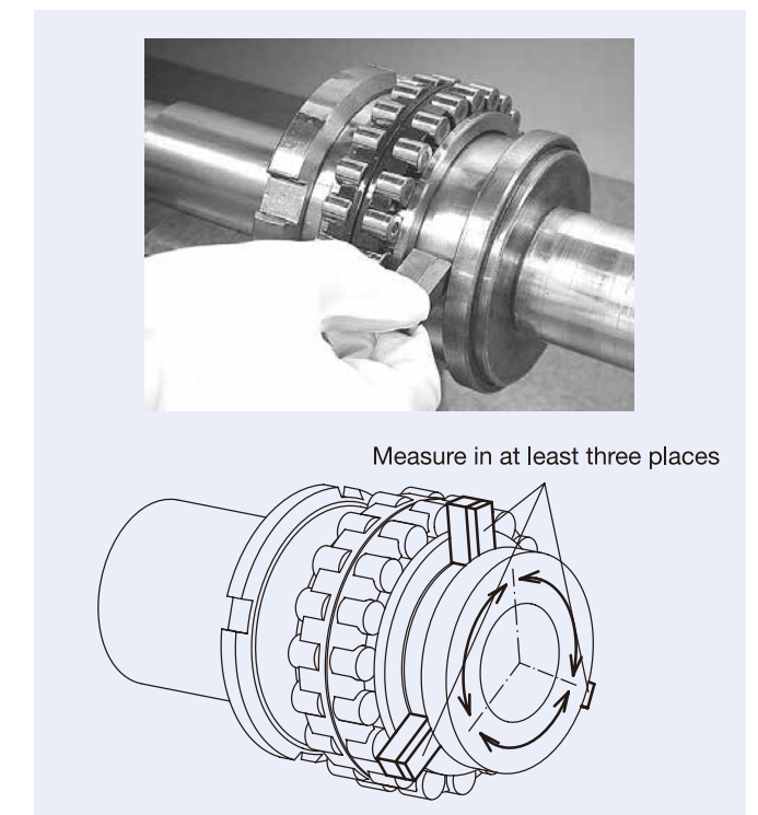
Fig. 1.6 Measuring the Required Spacer Width
