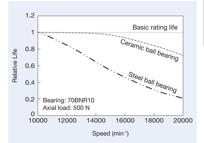
Fig. 1.8 Example Calculated Life Considering Centrifugal Force
