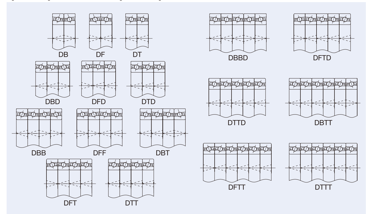
Fig. 3.12 Arrangements of Universal arrangement Bearings
