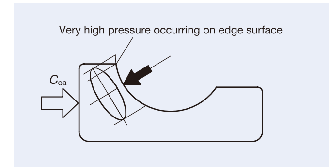
Fig. 2.3 C_{0a} and Limiting Axial Load
