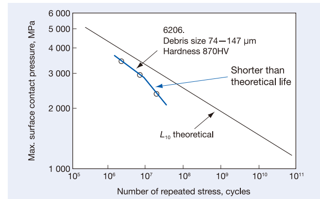
Fig. 1.3 Life Test Results Under Contaminated Lubrication Conditions
