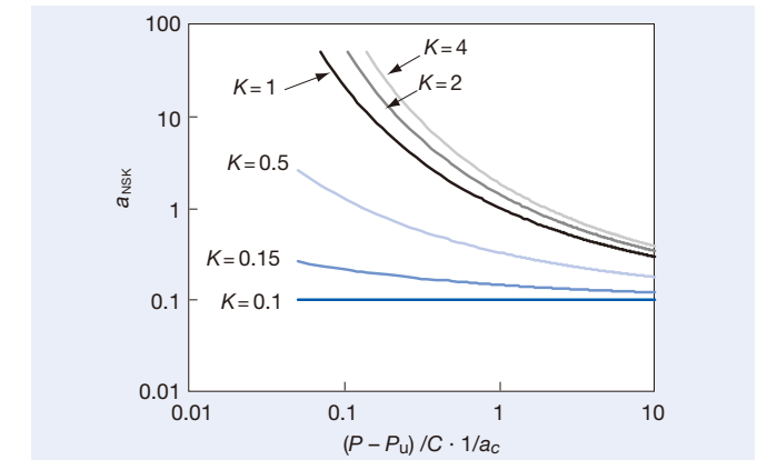
Fig. 1.5 New Life Calculation Graph for Roller Bearings
