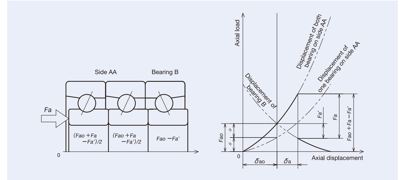
Fig 4.3 Axial Displacement in Position Preload (DBD Arrangement)
