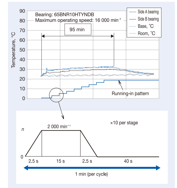
Fig. 3.3 Cycle Structure and Bearing Temperature Change during Intermittent Running-in
