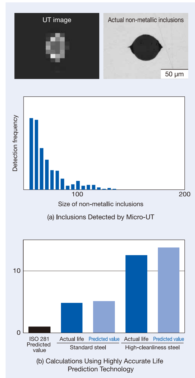
Fig. 1.6 Example Micro-UT Data and Life Prediction Results
