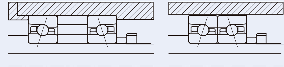
(a) Angular contact ball bearings in position preload
