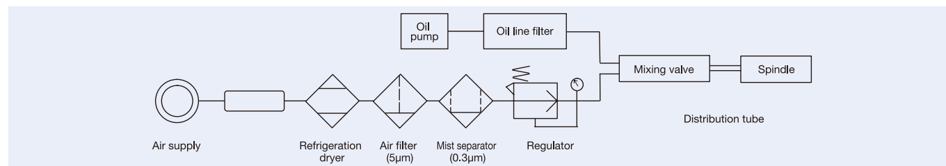
Fig. 6.4 Oil-Air Lubrication System (Example)
