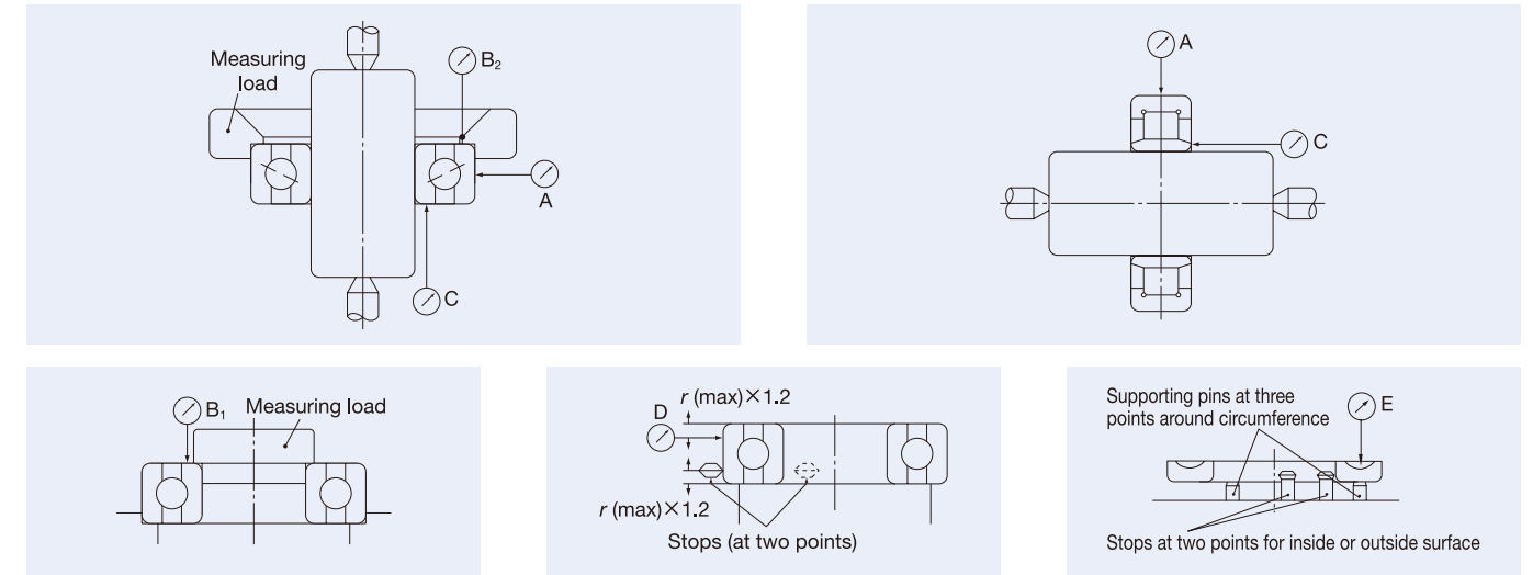
Fig. 7.1 Measuring Methods for Running Accuracy
