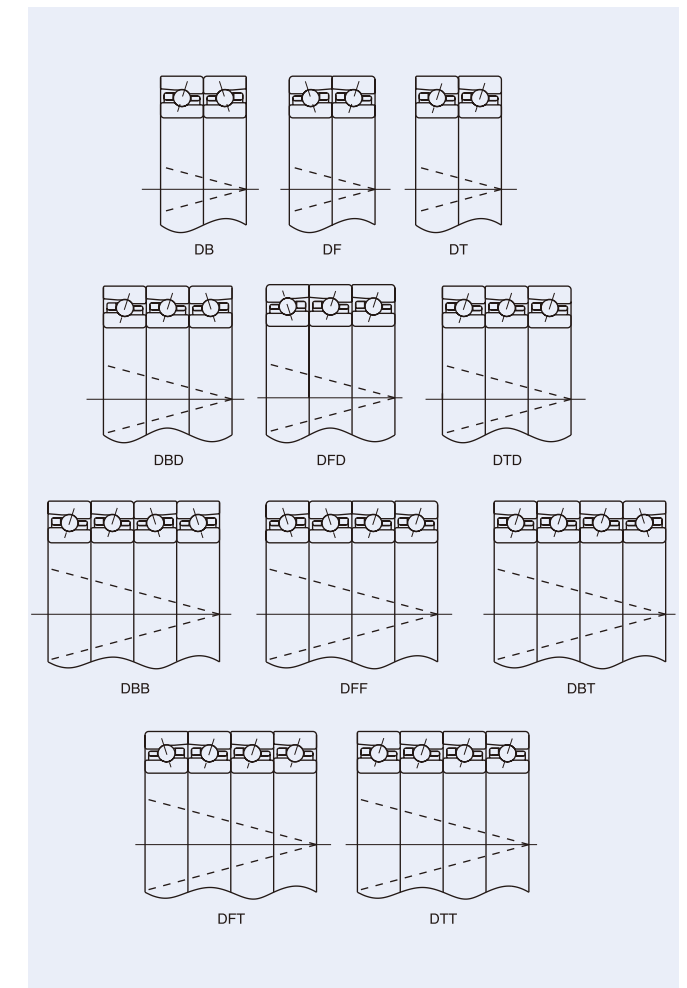
Fig. 3.6 Combinations of Angular Contact Ball Bearings
